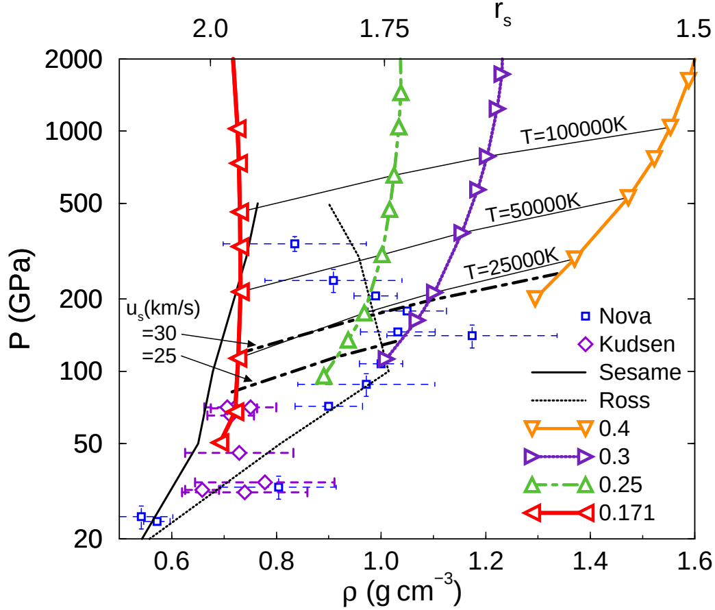
Figure 2. Pressure density diagram showing Hugoniot measurements [1, 3, 2] and results from chemical model calculations [4, 5] starting from the uncompressed liquid deuterium state ( \rho_0 = 0.171 \text{ g cm}^{-3} ). The triangles indicate Hugoniot curves from PIMC simulations for different initial densities \rho_0 given in the legend in units of \text{g cm}^{-3} . The thin solid lines are isotherms, the dash-dotted lines represent final shock states generated with the same shock velocity ( u_s = 25 and 30 \text{ km/s} ) starting from different initial compressions.
