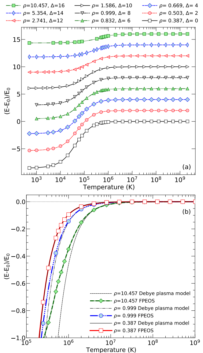
FIG. 3. Internal energy of hot, dense helium is shown for a collection of isochores. Their densities are given in units of \text{g cm}^{-3} . For clarity, we shifted the individual curves in the upper panel by \Delta and removed E_0 , the energy of a noninteracting Fermi gas of electrons and classical nuclei. In the lower panel, we show that the results from our first-principles simulation converge to prediction from the Debye plasma models in the limit of high temperature where screening effects are the dominant type of the interaction.
