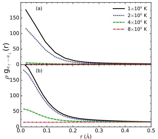
FIG. 14: The electron-electron pair-correlation functions for electrons with opposite spins in PIMC calculations of LiF plasma at densities of (a) 2.082 and (b) 15.701 \text{g cm}^{-3} (8-atom simulation cells).
