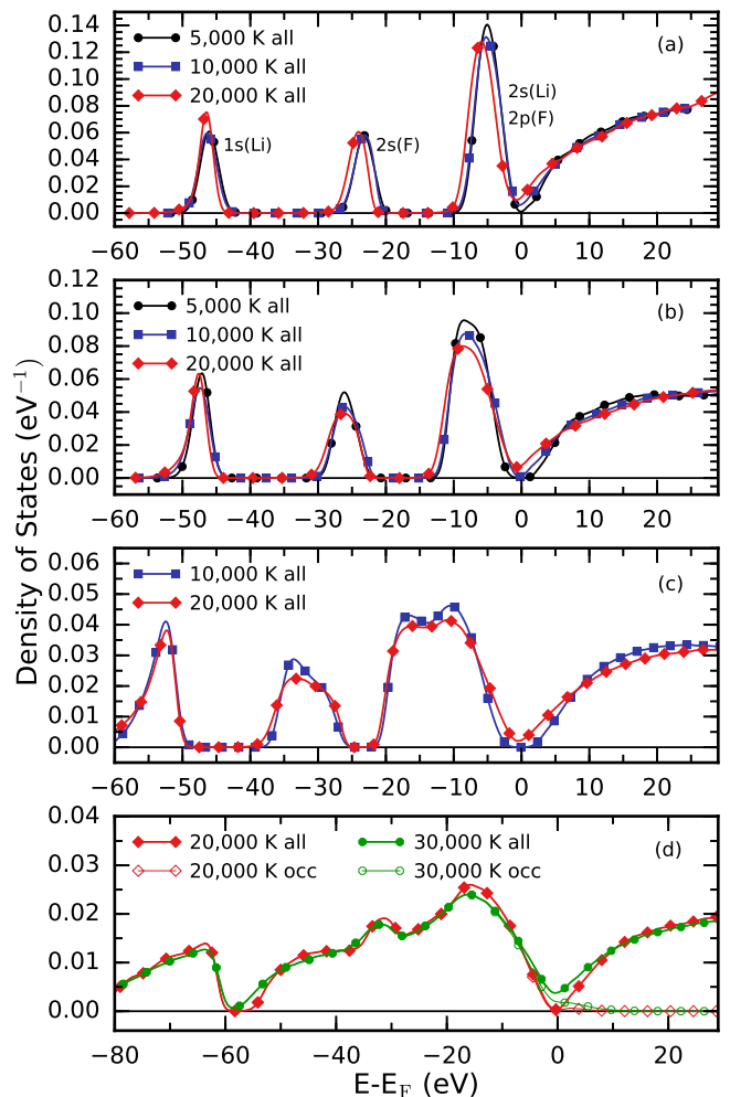
FIG. 17: Electronic DOSs at fixed, liquid temperatures at four densities of (a) 2.082, (b) 3.651, (c) 7.582, and (d) 15.701 g cm -3 .
