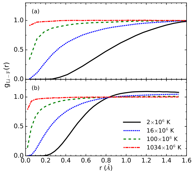
FIG. 10: Pair-correlation functions of Li-F nuclei computed with PIMC simulations of LiF over a wide range of temperatures at densities of (a) 2.082 and (b) 15.701 \text{g cm}^{-3} (8-atom simulation cells).
