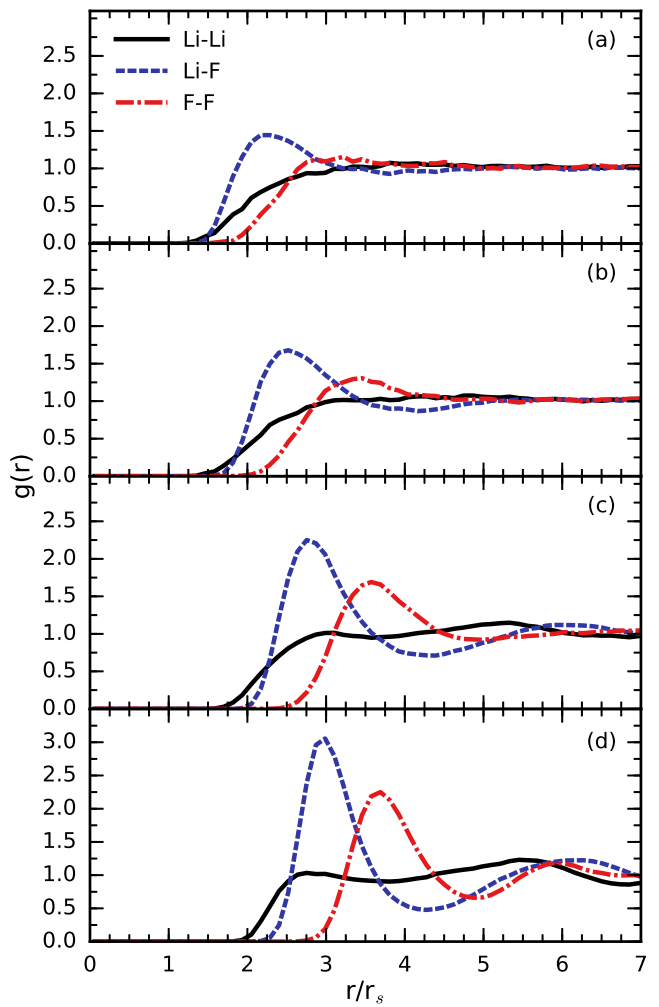
FIG. 7: Nuclear pair correlation functions for LiF liquid at a fixed temperature of 2 \times 10^4 K, computed with DFT-MD at four densities of (a) 2.082, (b) 3.651, (c) 7.582, and (d) 15.701 \text{g cm}^{-3} (8-atom simulation cells).
