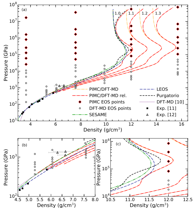
FIG. 1: (a) Comparison of PIMC/DFT-MD shock Hugoniot curves with SESAME (7271) 4,5 , LEOS (2240) 6-8 , and Purgatorio (Lynx 2240) 9 models, as well as previous DFT-MD 10 and experiments 11,12 in P - \rho space. The PIMC/DFT-MD Hugoniot curves are plotted for four initial densities, corresponding to 1–1.3-fold of ambient density. PIMC/DFT-MD and Purgatorio treat the quantum-mechanical shell structure of the ions and, thus, reveal a pronounced compression maximum and a shoulder due to K-shell and L-shell ionization effects. SESAME and LEOS do not treat shell effects and, thus, predict the overall behavior without shell effects. Plots (b) and (c) show a zoom in of the regions near the experimental data and the compression maximum, respectively.
