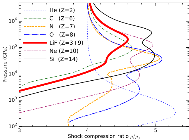
FIG. 6: Comparison of shock Hugoniot curves in P - \rho/\rho_0 space for various materials initialized at ambient or experimental densities. The initial densities (in \text{g cm}^{-3} ) are He: 0.124, C: 2.253, N 0.807, O: 0.667, LiF: 2.635, Ne: 1.507, and Si: 2.329.
