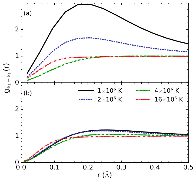
FIG. 15: The electron-electron pair-correlation functions for electrons with parallel spins in PIMC calculations of LiF plasma at densities of (a) 2.082 and (b) 15.701 g cm -3 (8-atom simulation cells).
