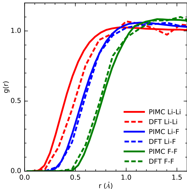
FIG. 11: Comparison of nuclear pair-correlation functions for LiF at a temperature of 1 \times 10^6 K and a density of 15.701 \text{ g cm}^{-3} computed with PIMC and DFT-MD (24-atom simulation cells).
