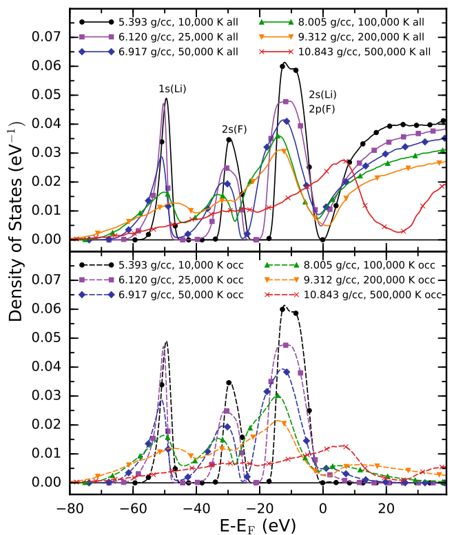
FIG. 16: Electronic DOS plotted at temperature-density conditions along the principal shock Hugoniot curve. The upper panel shows the total DOS (all), while the lower panel shows the occupied DOS (occ).
