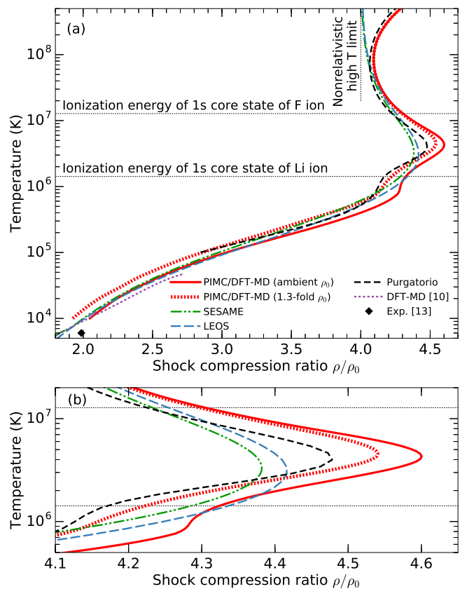
FIG. 5: (a) Comparison of PIMC/DFT-MD shock Hugoniot curves with SESAME (7271) 4,5 , LEOS (2240) 6-8 , and Purgatorio (Lynx 2240) 9 models, as well as previous DFT-MD 10 and experiments 13 in T - \rho/\rho_0 space. The PIMC/DFT-MD Hugoniot curves are plotted for two initial, pre-compressed density states, corresponding to 1-fold and 1.3-fold of ambient. As in Fig. 1, PIMC/DFT-MD and Purgatorio predict shell structure effects along the Hugoniot, while SESAME and LEOS predict the overall behavior without shell effects. Plot (b) shows a zoom in of the compression maximum region.
